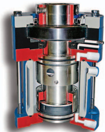
Double Mechanical Seal
